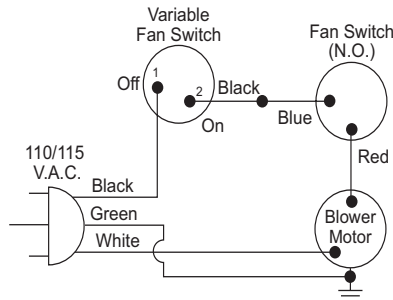
Figure 11: Wiring Diagram (BKT Model Only)
